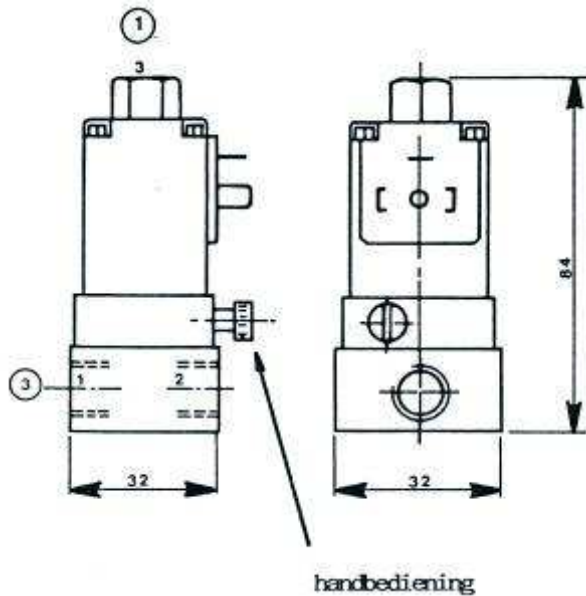
3/2-Way solenoid valve
