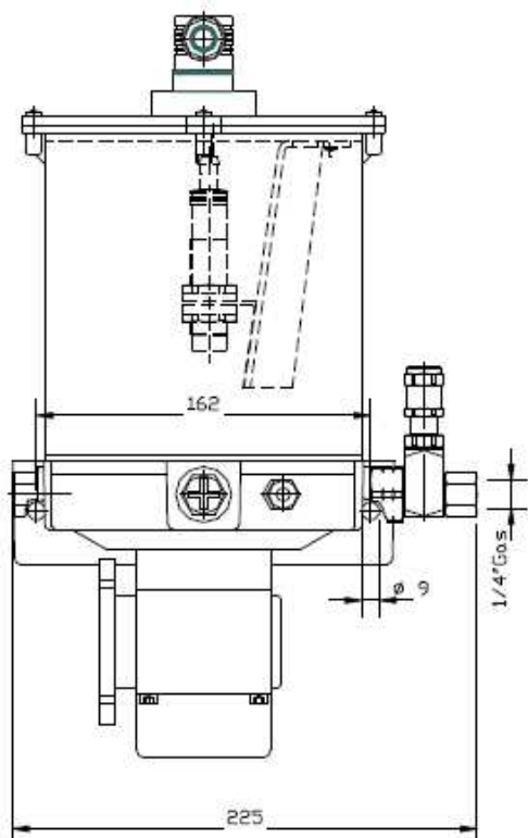
OVERALL DIMENSION
